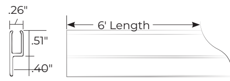
Mounting Channel
