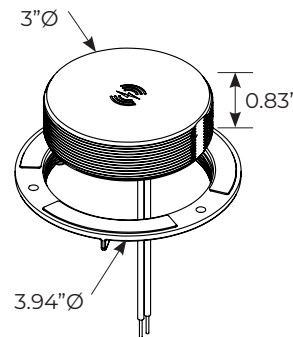
Under mount
