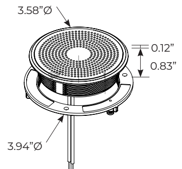
Surface mount
