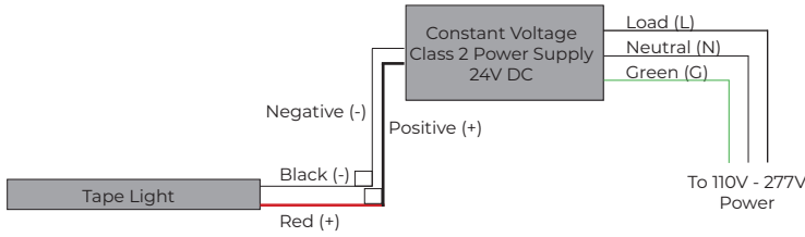
Single Color Wiring
