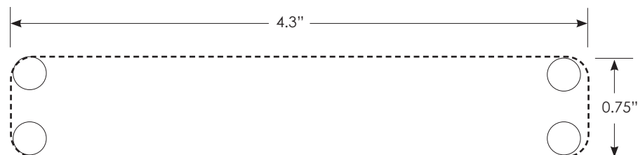
Cutting Template
